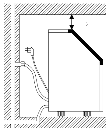
Side view (inch)
