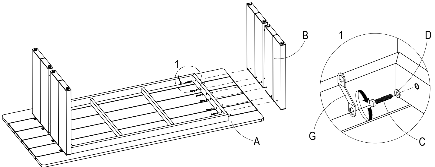
C= Hexagonal bolt (12 pcs)
