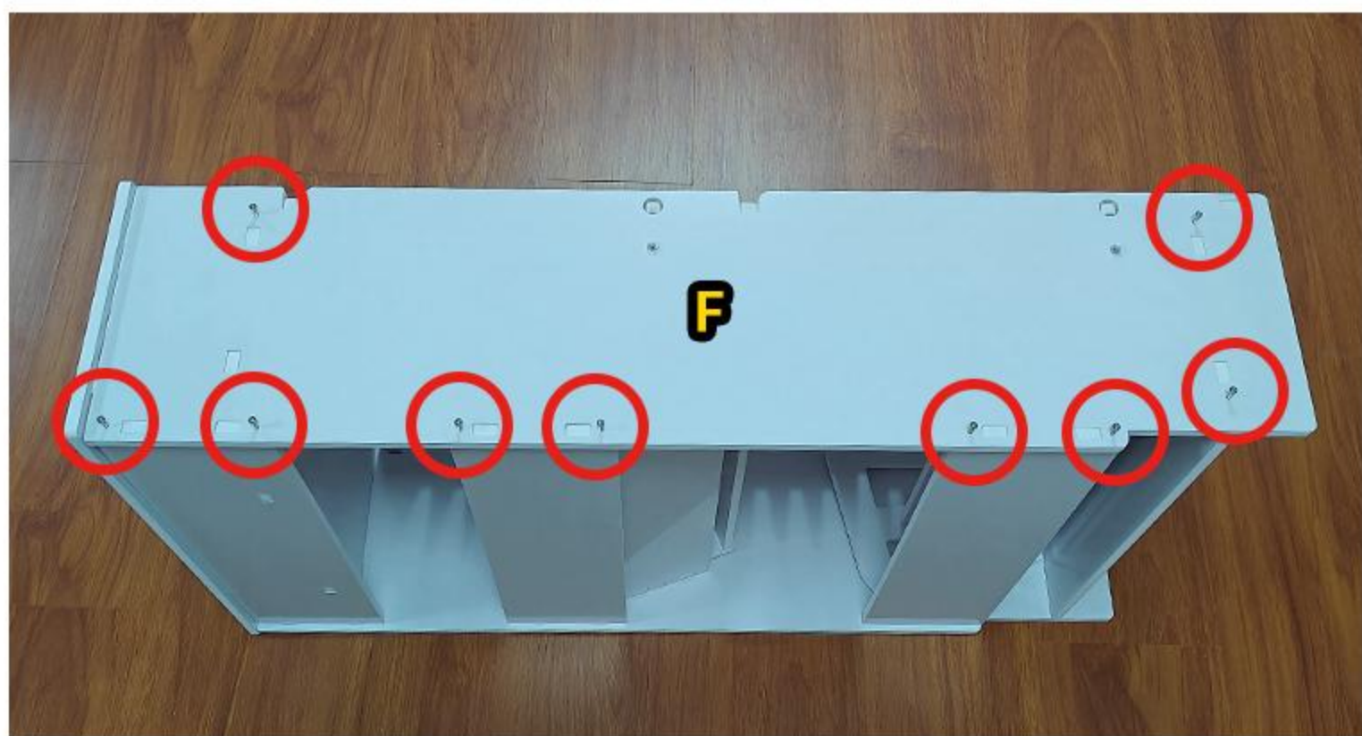
21.INSTALL NINE LONG SCREWS ON EACH OF THE TWO F-PLATES; WE NEED A TOTAL OF EIGHTEEN PIECES
