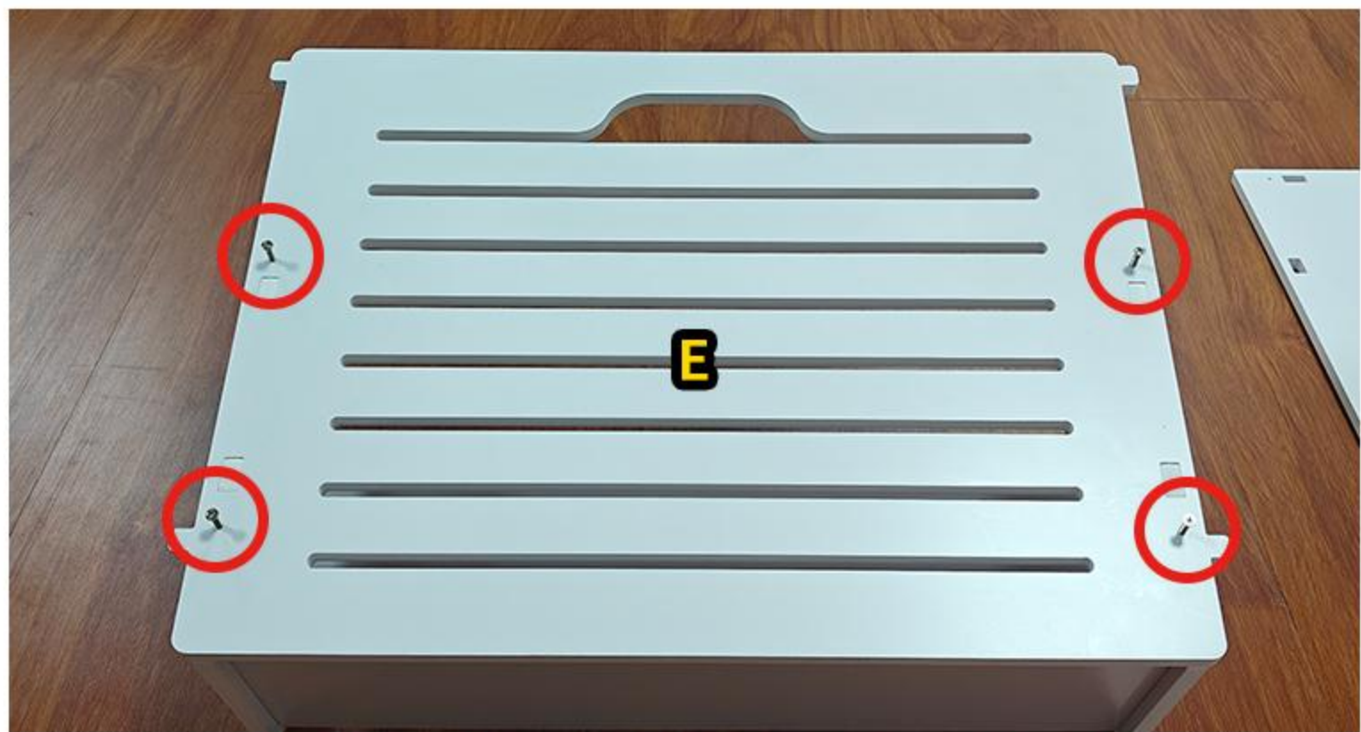
9.TIGHTEN THE FOUR LONG SCREWS ON BOARD E
