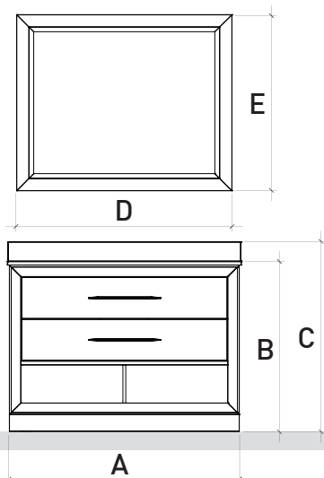
FRONT VIEW VUE DE FACE VISTA FRONTAL
