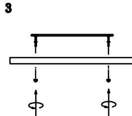
Fix the lamp body to the ceiling
