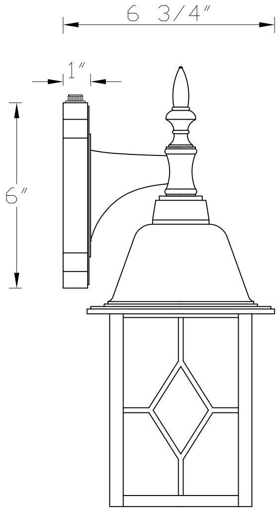
SIDE VIEW
