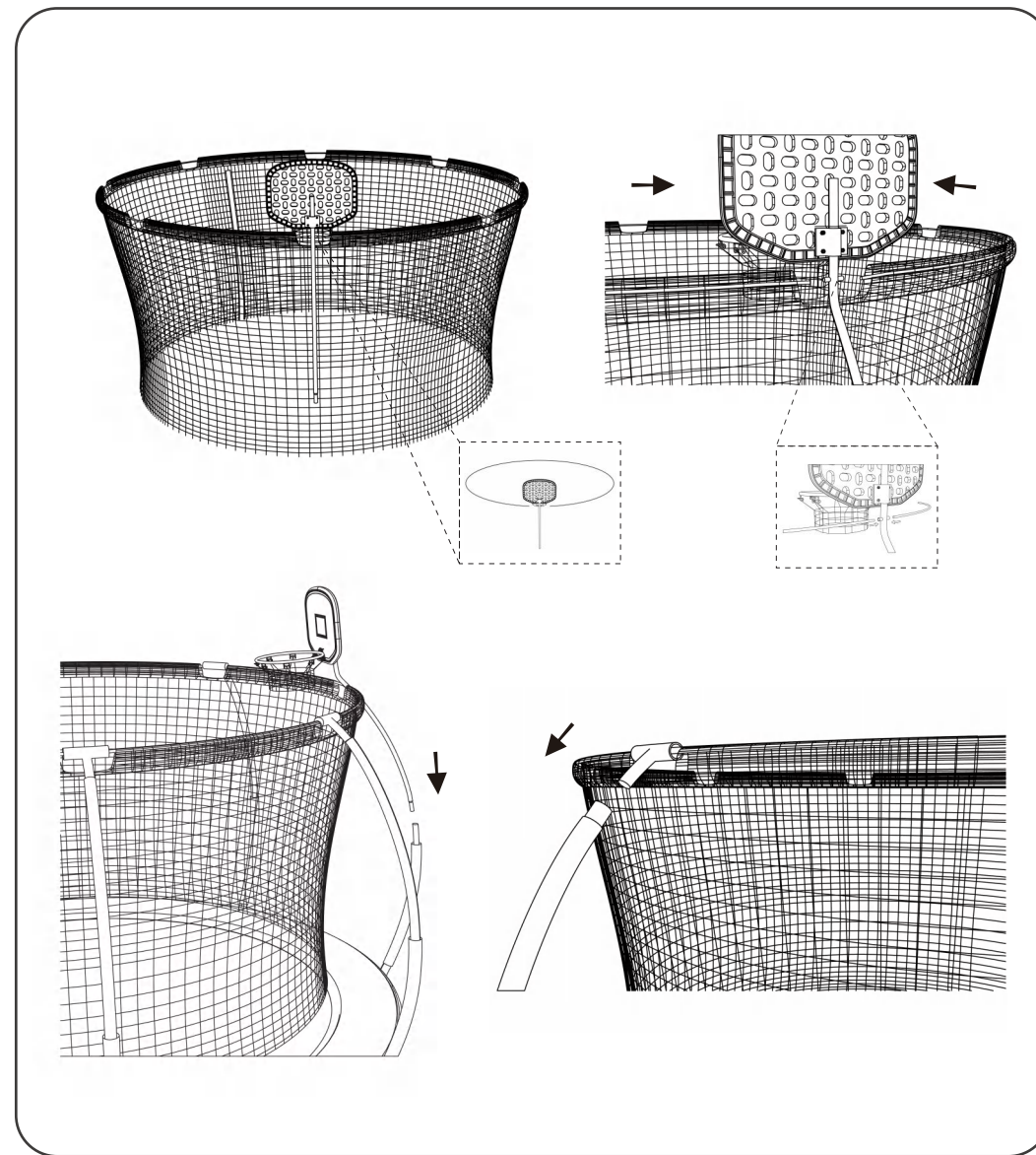
Step 10. Connect the longer upper net pole to the lower net pole, and then install the safety enclosure net by inserting the T-shaped connectors for the carbon fiber rod into the upper net poles.
