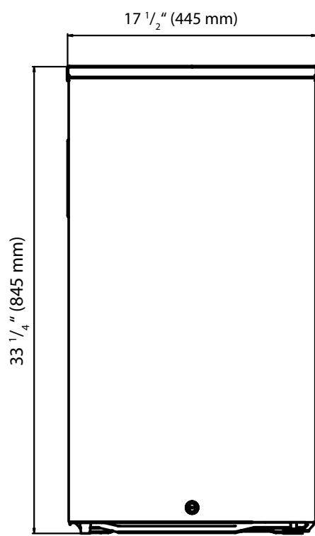
Front View
