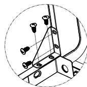
M6x13 Screw Qty: 4 pcs
