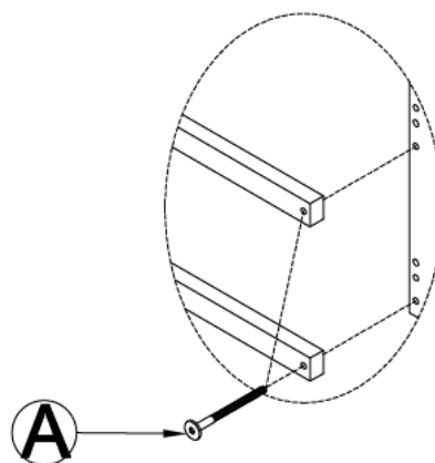
Detail 2
