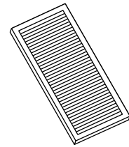
F-310X165X12mm(1pc)
