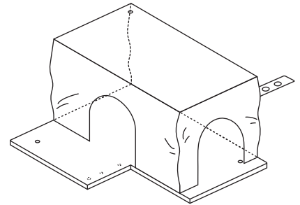
C-540X440X12mm(1pc)
