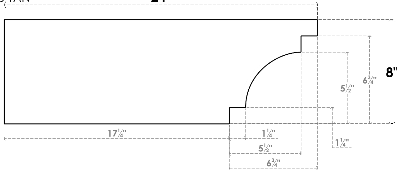
SIDE PROFILE
