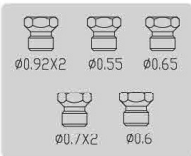
Nozzles for LPG (7)
