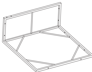
C 1pc (Seat Panel)
