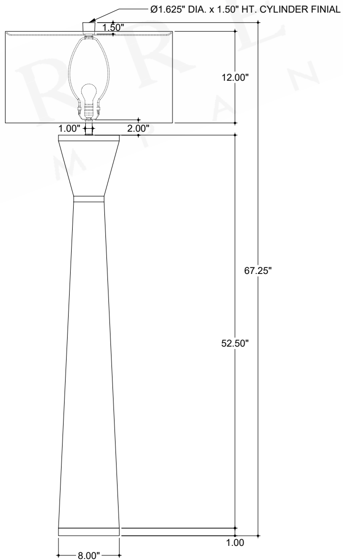
FRONT VIEW
