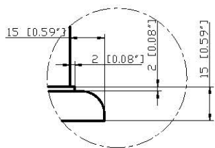
A DETAIL 4:1
