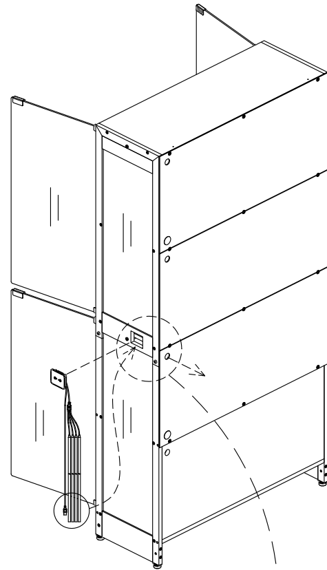
VIEW-B
