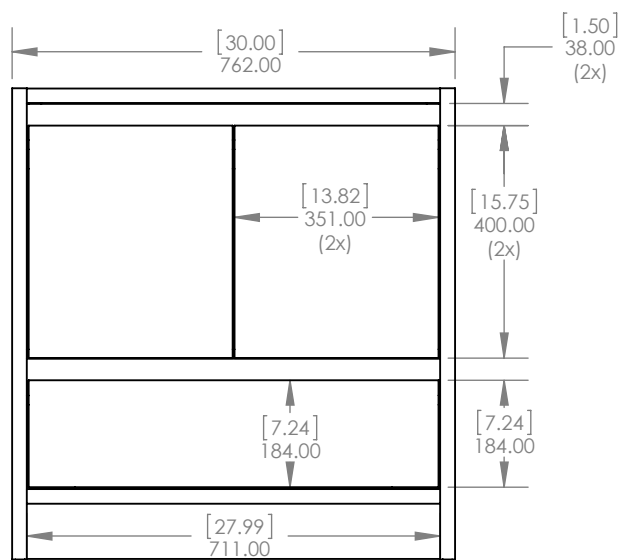
Front view / Vista Frontal
