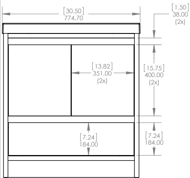
Front view / Vista Frontal
