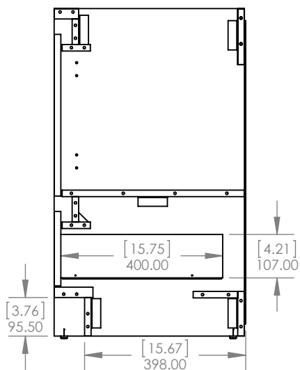
Side View / Vista Lateral
