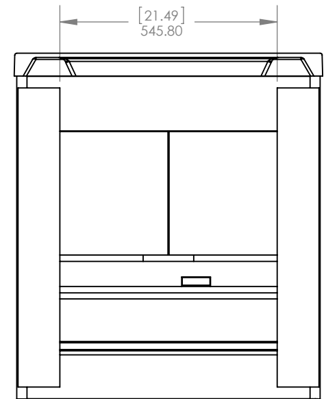
Back View / Vista Trasera
