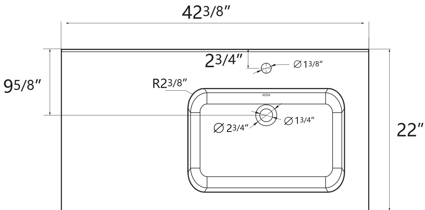
Top View
