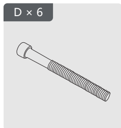
M8x70mm Screws
