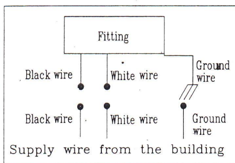
Circuit diagram 1
