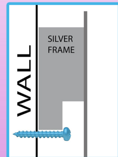
Lip for hanging over screws
