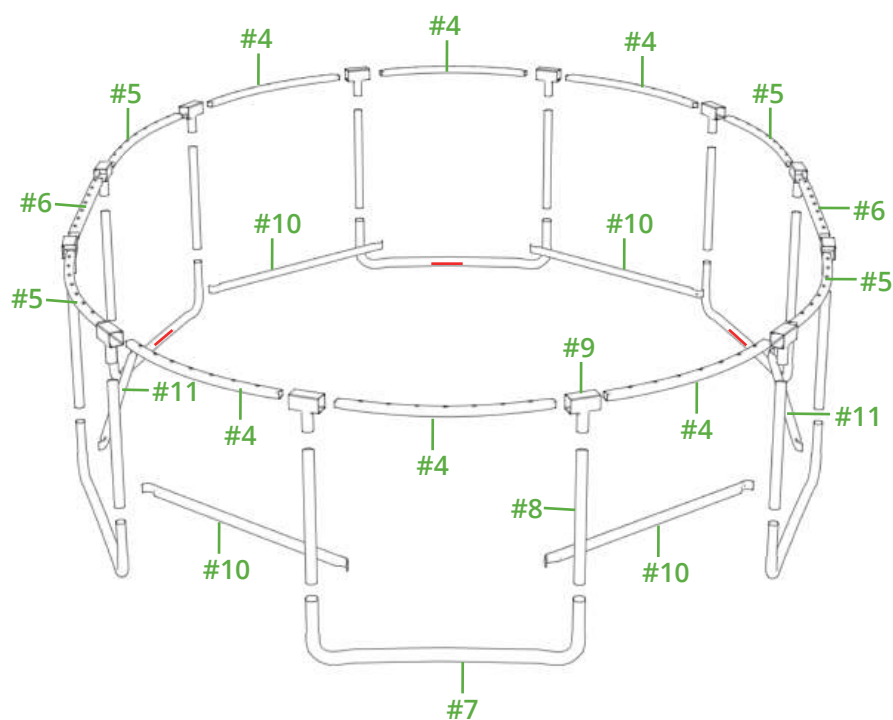
Frame Installation Example Diagram
