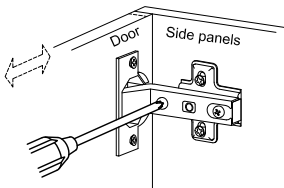
Horizontal by screw adjustment
