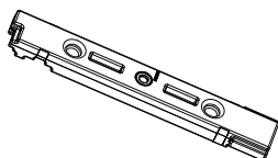
P90143-3 RIGHT CONNECTING POST 1 PC(S)
