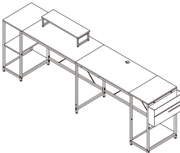
Design C: Straight Long Desk
