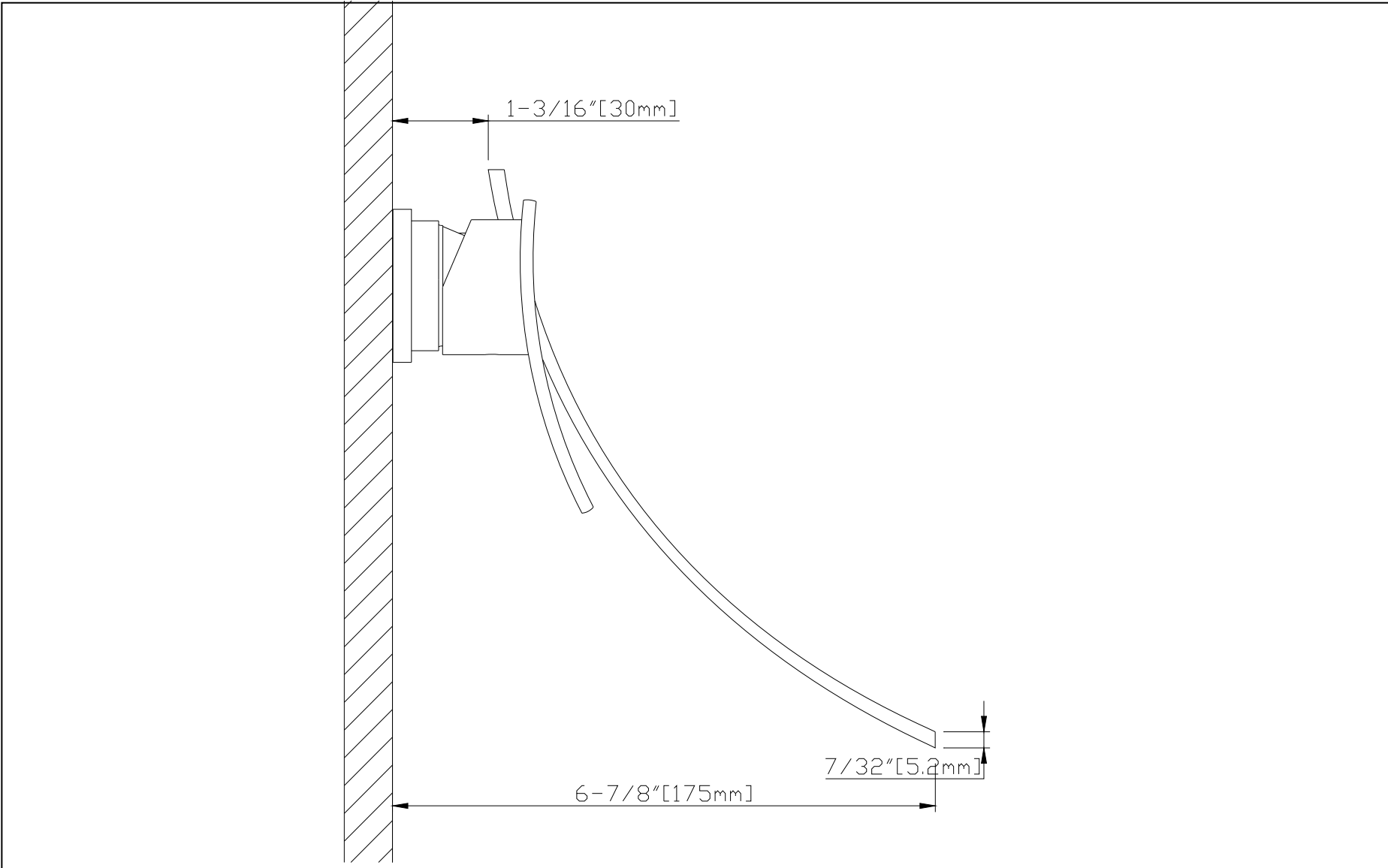
RIGHT SIDE VIEW OF FAUCET
