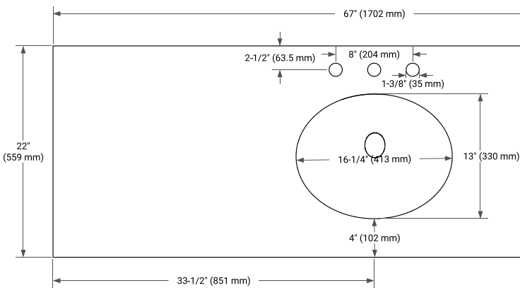
COUNTERTOP PLAN VIEW
