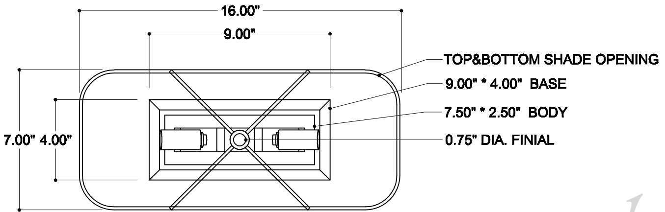
TOP VIEW
