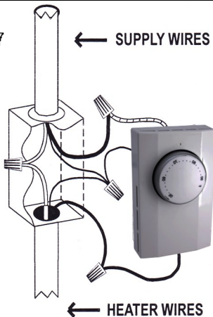
Connection Diagram for Wall Mounted Single Pole Thermostat
