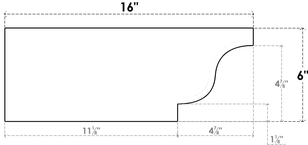
SIDE PROFILE
