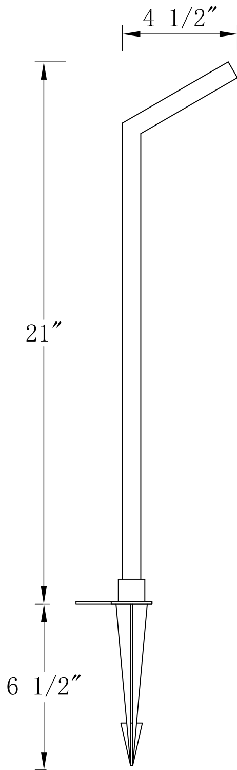
FRONT VIEW
