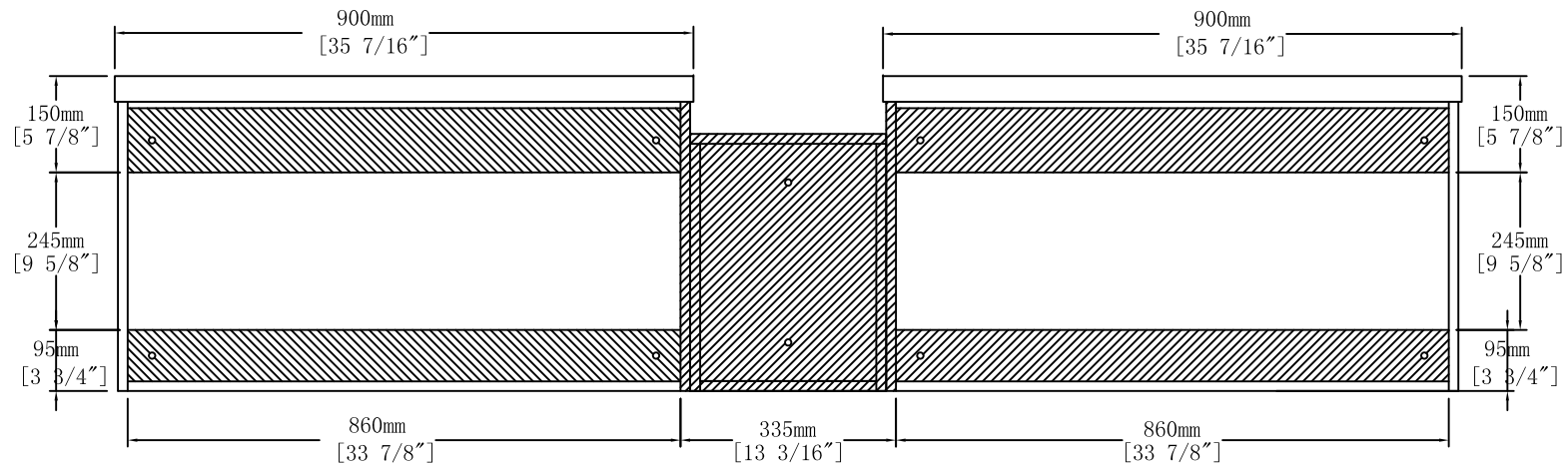
Back View
