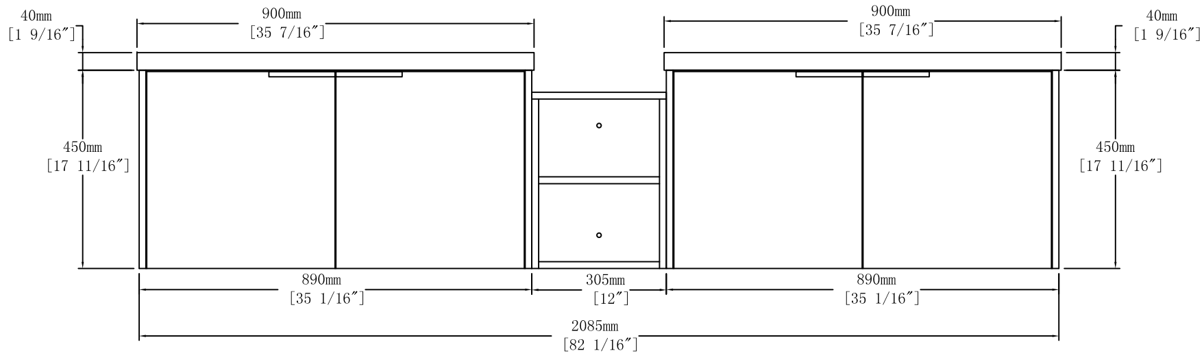
Front View
