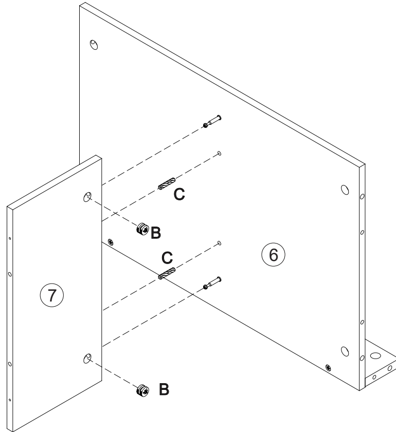
Cam Lock Fastening System
