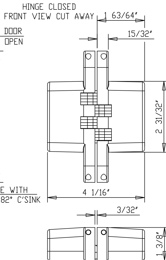
HINGE CLOSED TOP VIEW CUT AWAY
