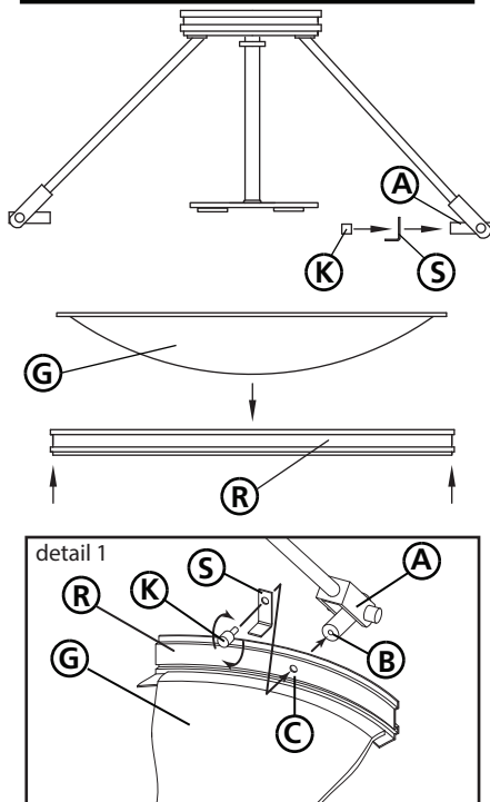
Drawing 3 - Fixture Mounting
