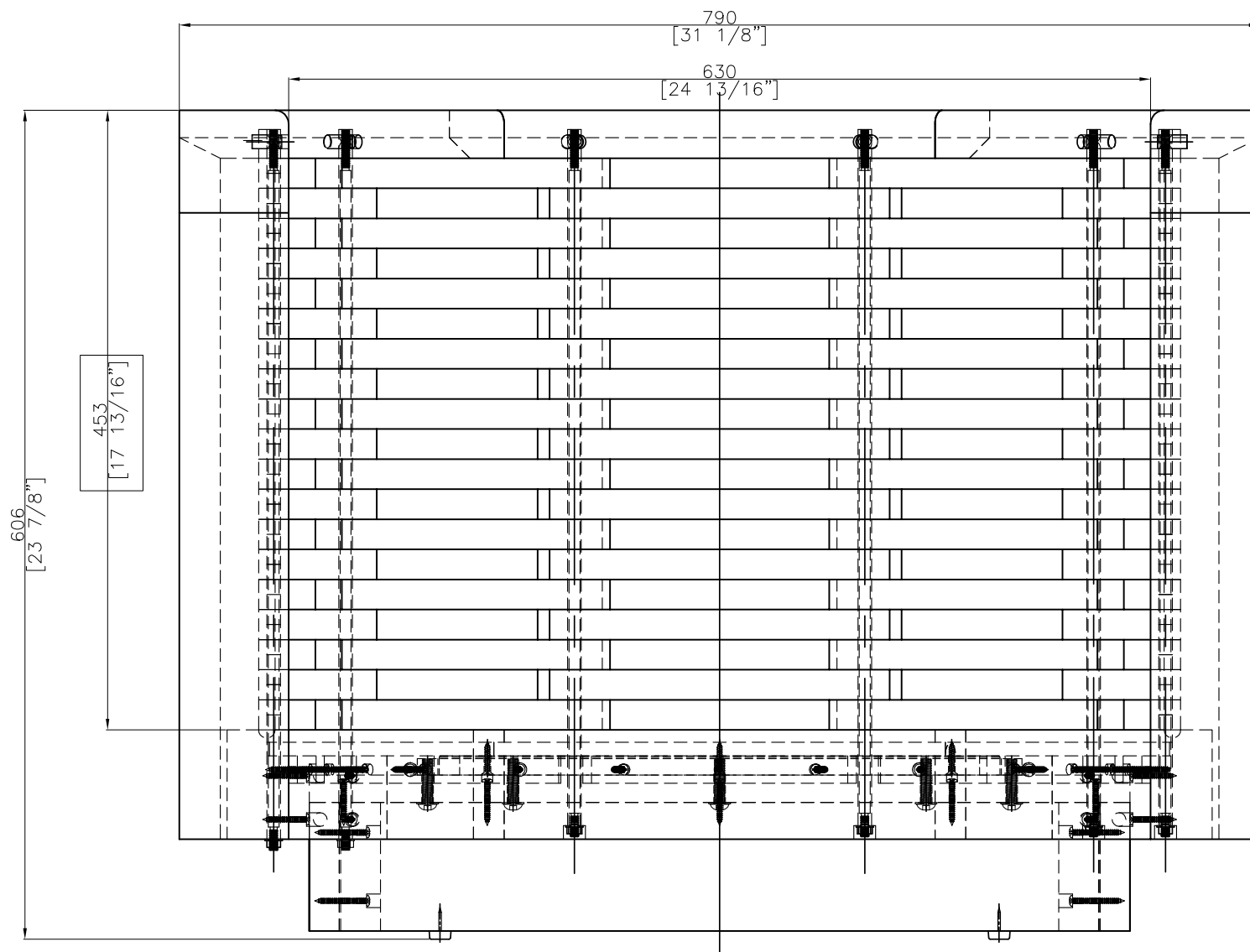
FRONT VIEW
