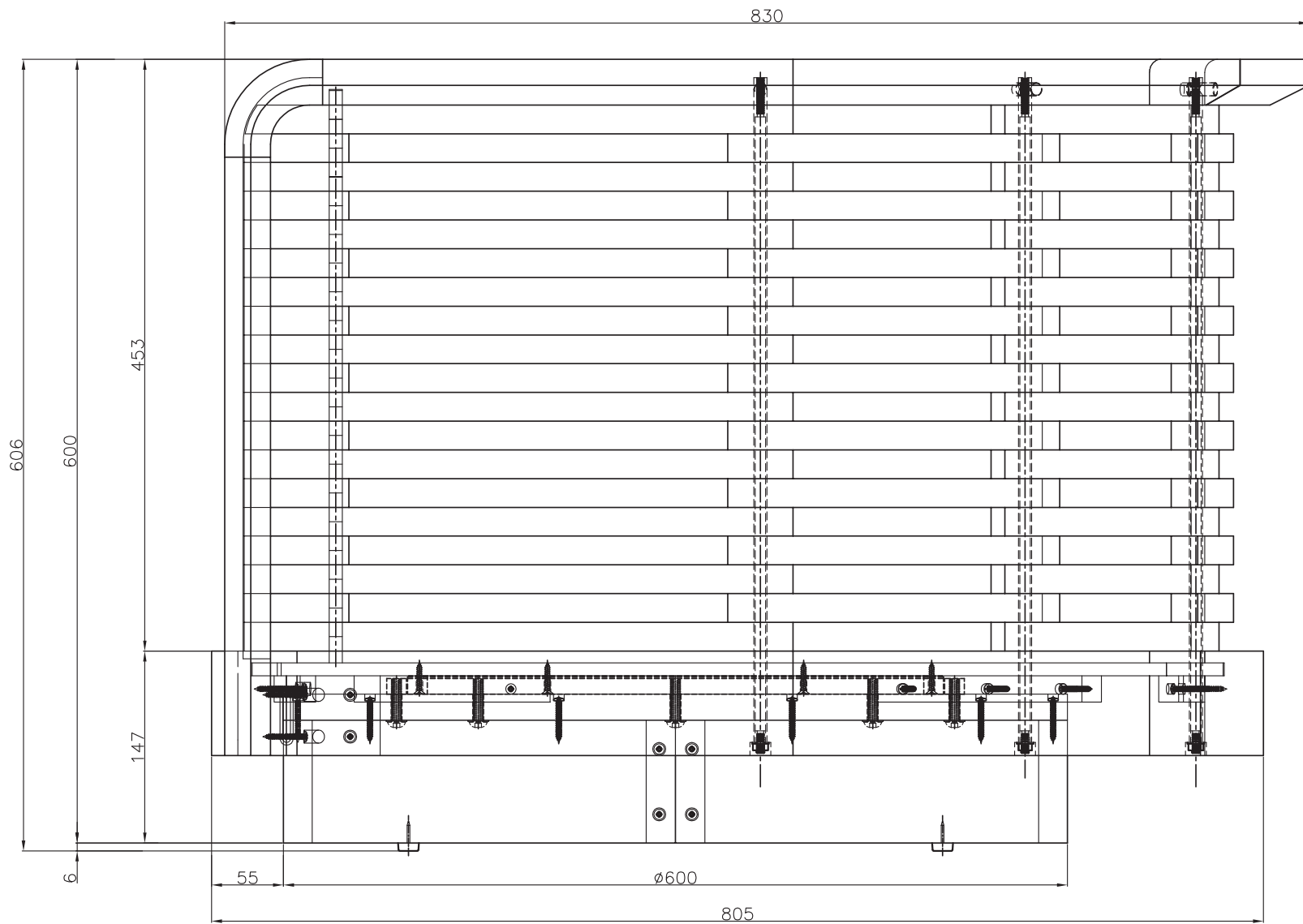
SIDE VIEW
