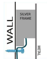
Wall mount detail
