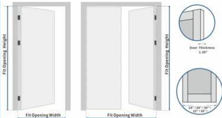
Interior Door Rough Opening Guide
