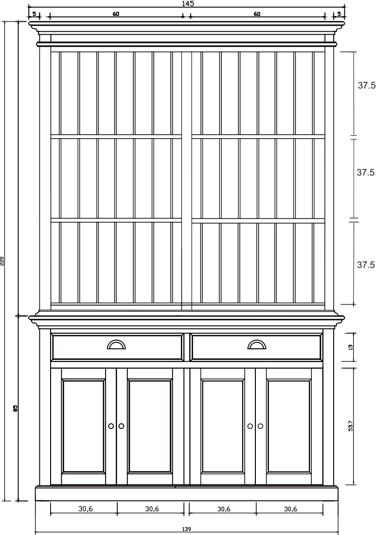
FRONT VIEW
