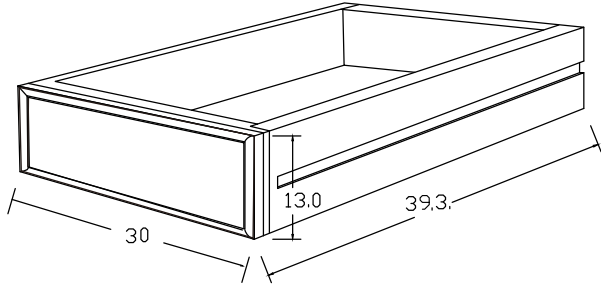
DETAIL DRAWER SMALL
