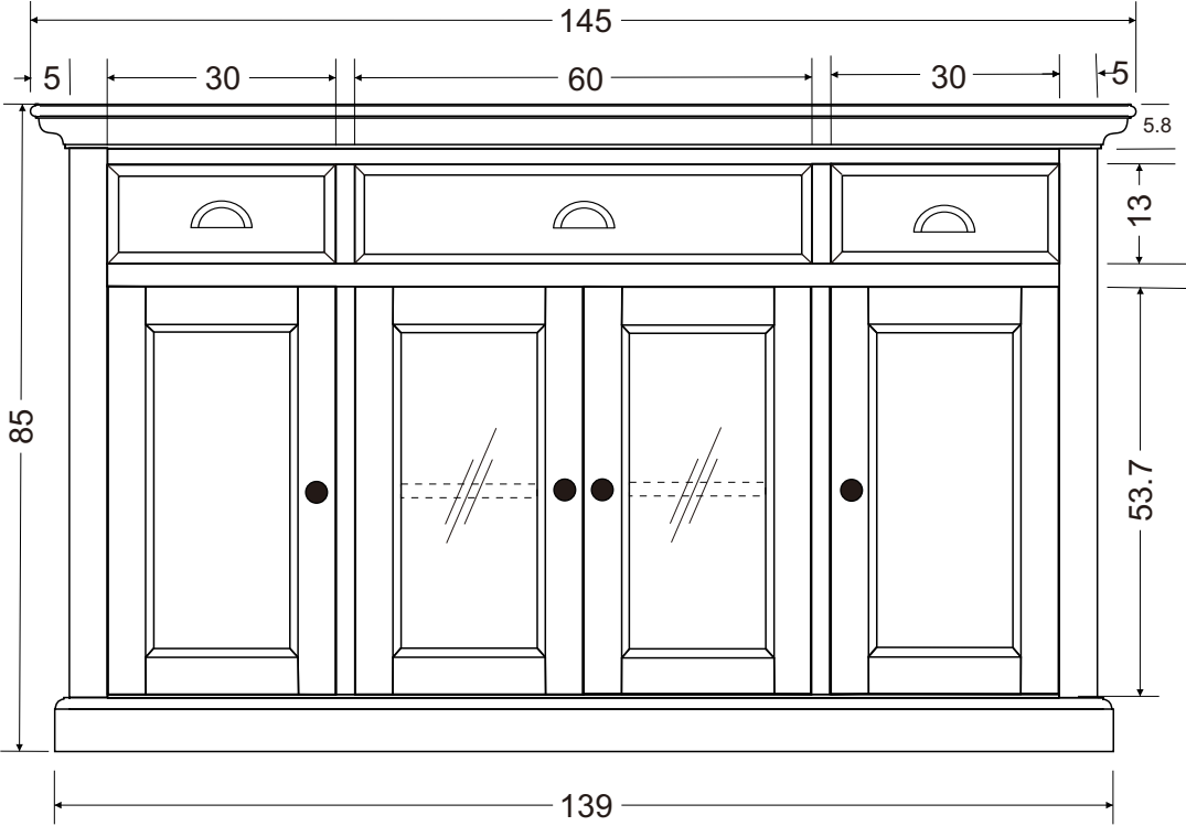
FRONT VIEW
