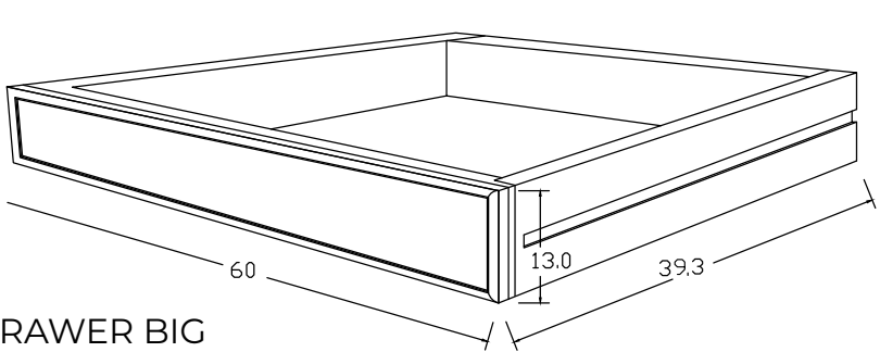
FRONT OPEN VIEW
