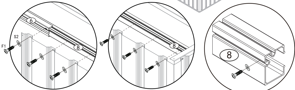
Screw mounting position
