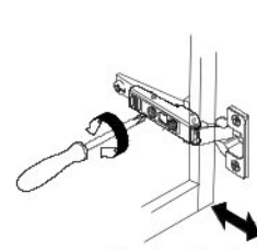
Depth adjustment
