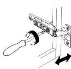
Side adjustment
