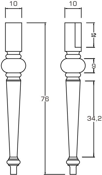
LEG DETAIL
