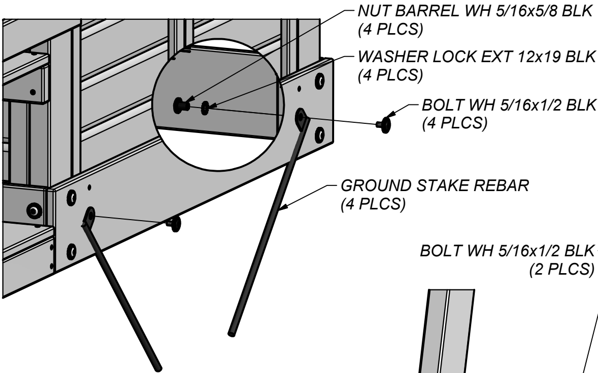
FORT GROUND STAKES
