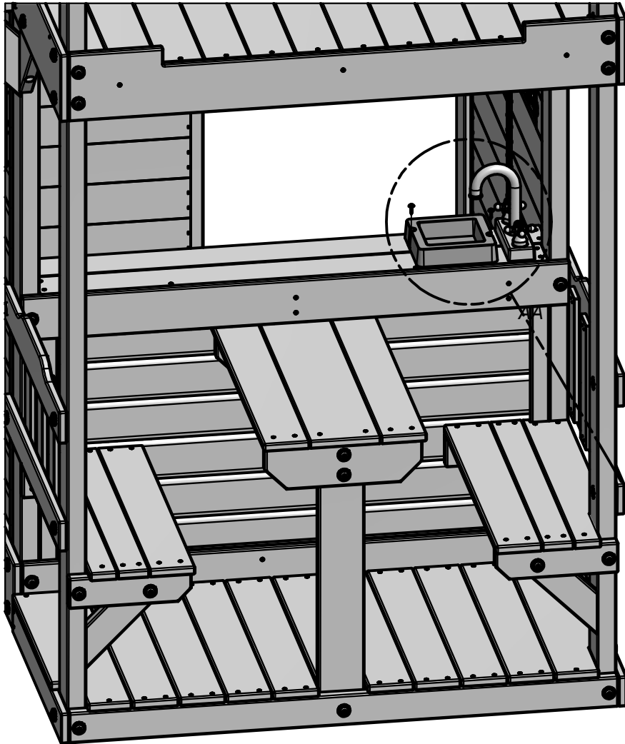
SCREW PWH 8x5/8 (2 PLCS)
