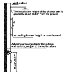
2.23 From ground to main body usually 35.43-39.37 inches also can according to user height or user demand.
