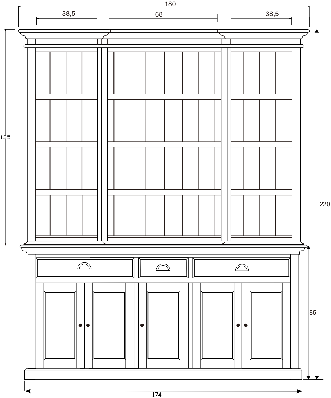
FRONT VIEW
