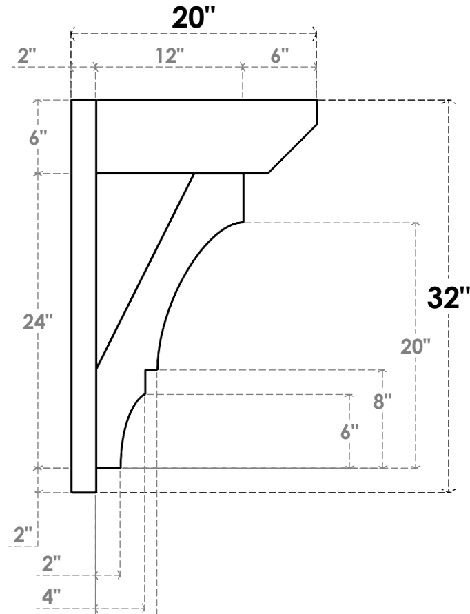
SIDE PROFILE
