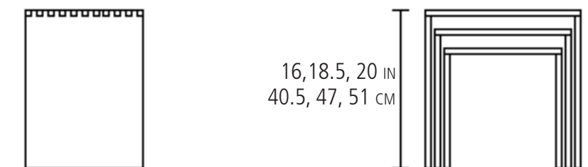
ELEVATIONS
