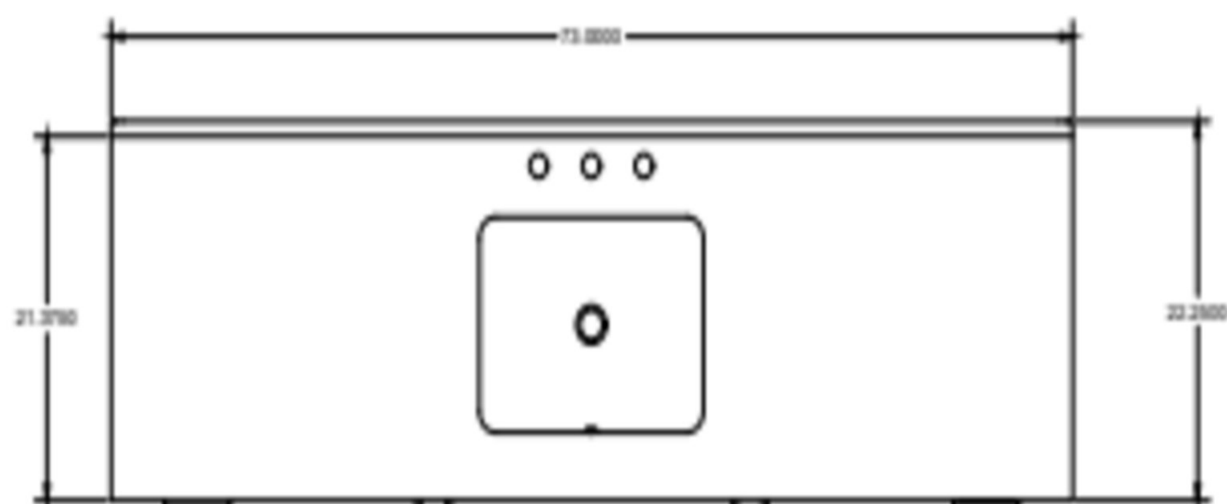
TOP VIEW
